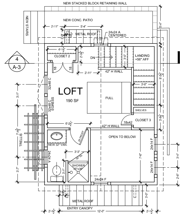
3 PROPOSED LOFT PLAN
