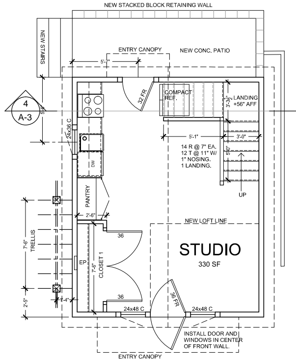
2 PROPOSED FLOOR PLAN
