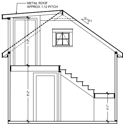
4 PROPOSED SECTION
