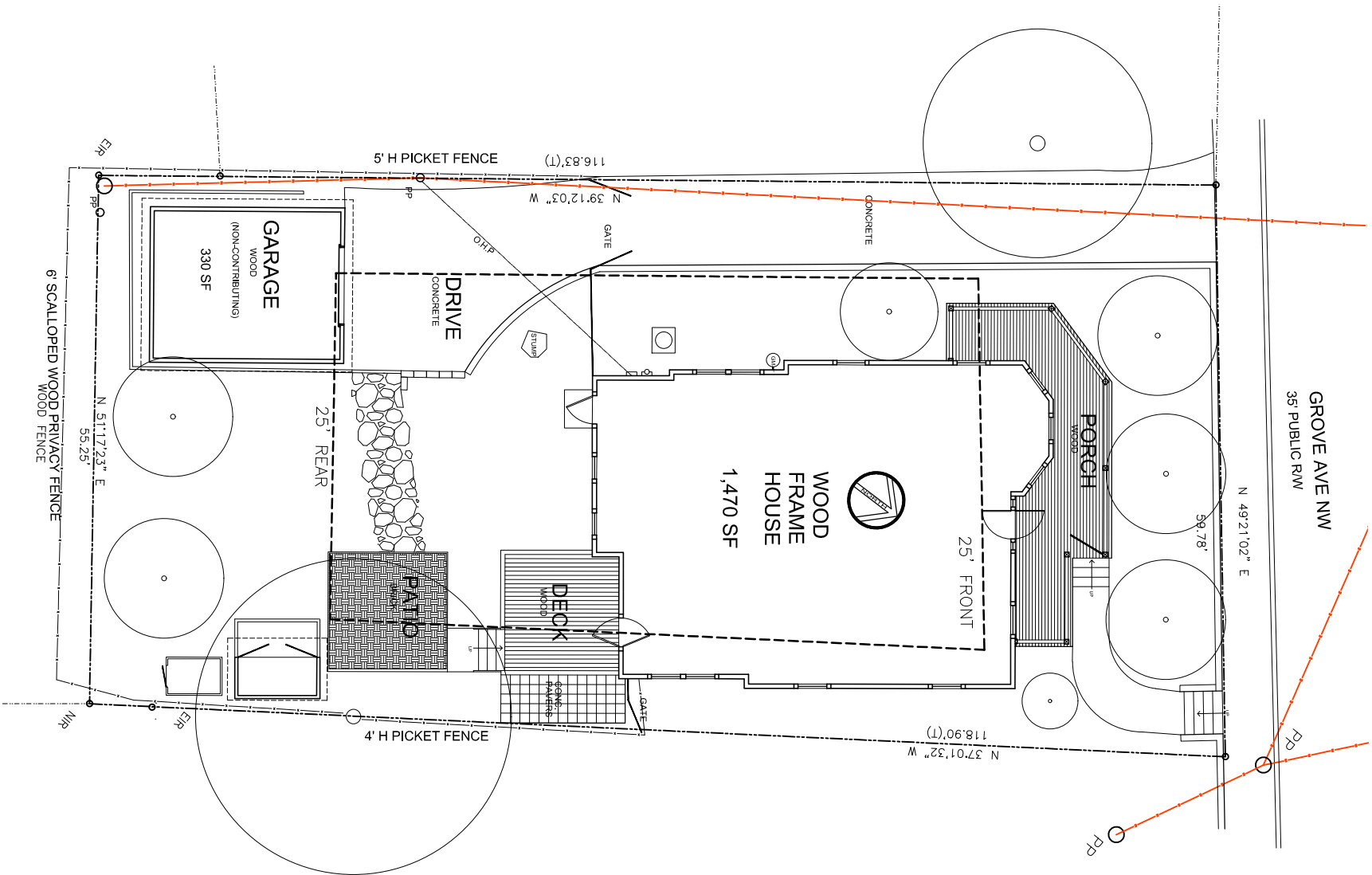
1 EXISTING SITE PLAN A-1 1/16" = 1'-0" 1,470 SF - FOOTPRINT 0.156 ac
